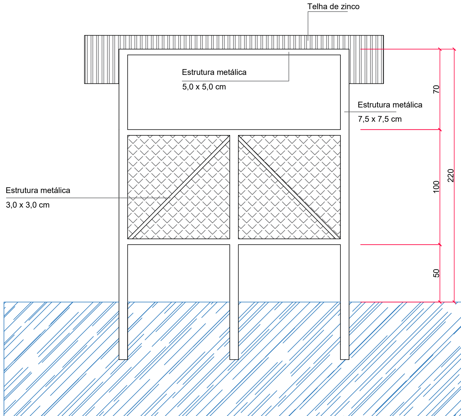
Vista frontal
